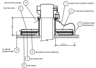
G2 GREASE GUARD SPECIFICATION SECTION VIEW AT CENTER OF CURB
