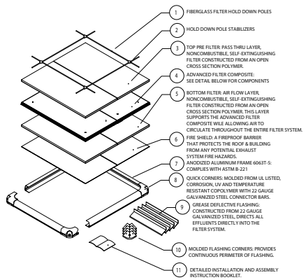
G2 GREASE GUARD SPECIFICATION CUT-AWAY VIEW
