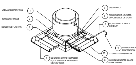
G2 GREASE GUARD SPECIFICATION CUT-AWAY VIEW
